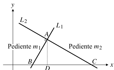
Figura P.17 \triangle ABD es similar a \triangle CAD .
