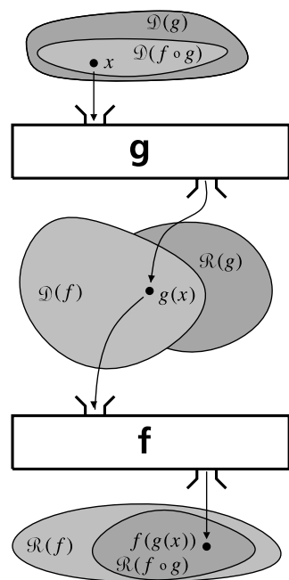
Figura P.57 f \circ g(x) = f(g(x)) .
