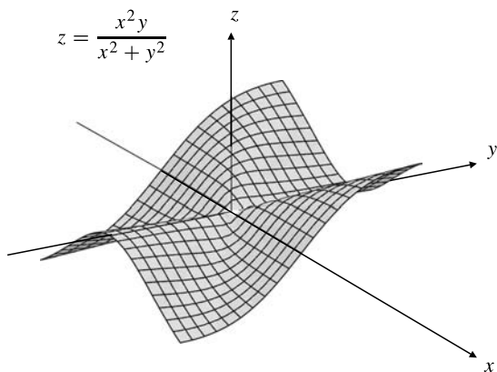
Figura 12.14 \lim_{(x, y) \rightarrow (0, 0)} \frac{x^2y}{x^2 + y^2} = 0.
