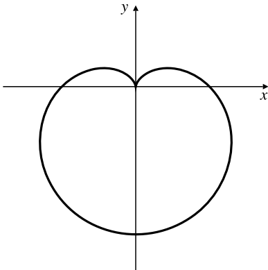
Figura 8.39 La cardioide r = a(1 - \sin \theta) .
